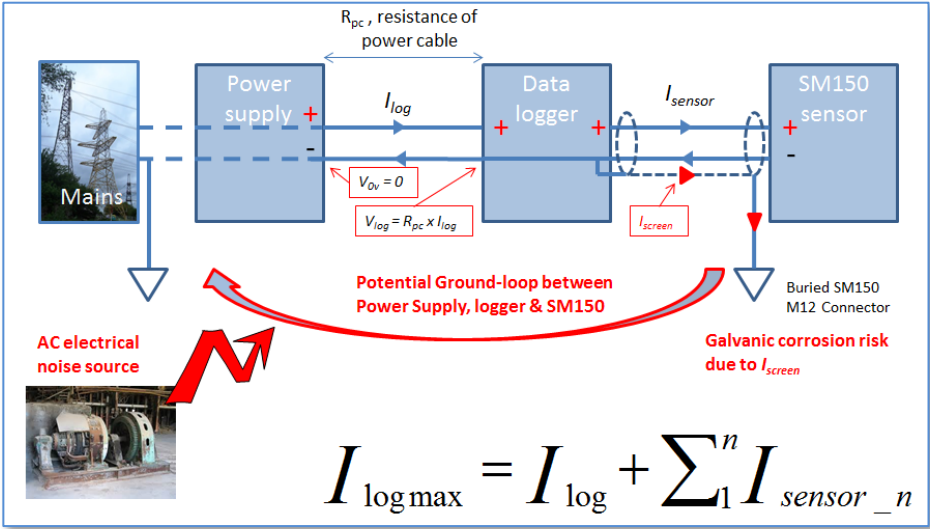
Figure 2 This diagrams shows that if the logger is are not well grounded then a potential ground loop can exist between the sensor and the power supply and/or mains power, and also the risk of galvanic corrosion to buried M12 connectors on the sensor and cable.
